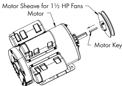
1 1/2 HP Motor with 2 Set Screw Sheave
