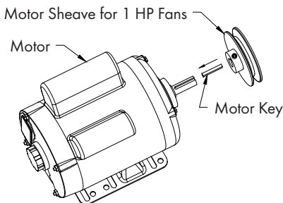
1 HP Motor with 1 Set Screw Sheave
