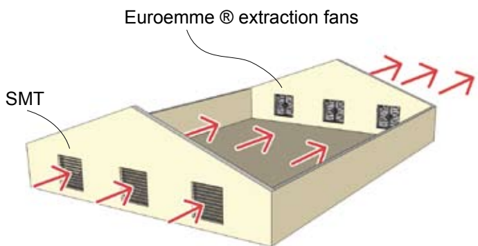
SMT shutters functioning in combination with Euroemme® extraction fans.
