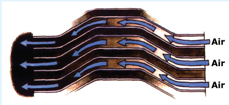
The gentle bends are the key to MI-T-Dark light trap performance
