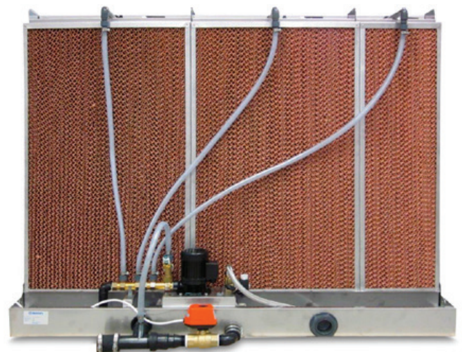
GX40 media assembled in Munters FA6 humidifier.
