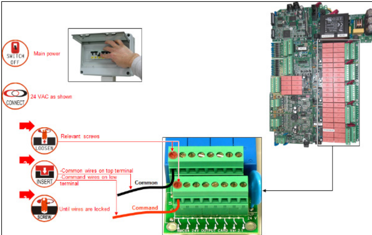
24VAC OUTPUT CARD CONNECTION- EXAMPLE
