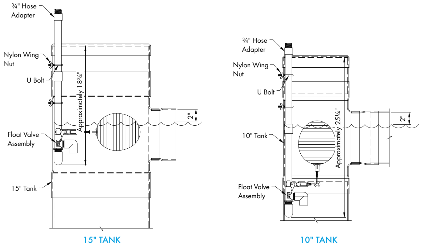
Figure 22E COMPLETED ASSEMBLY
