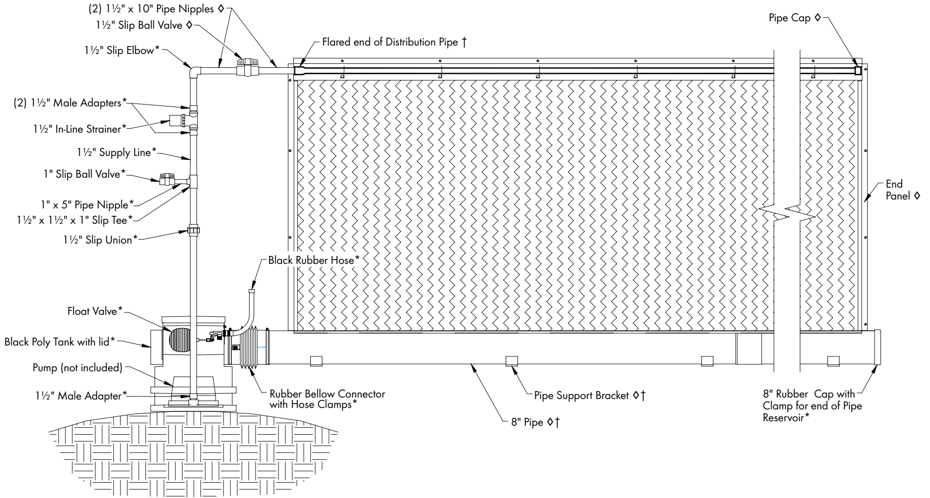
Figure 24 EC1642 BLACK POLY TANK ELEVATION VIEW WITH SUBMERSIBLE PUMP
