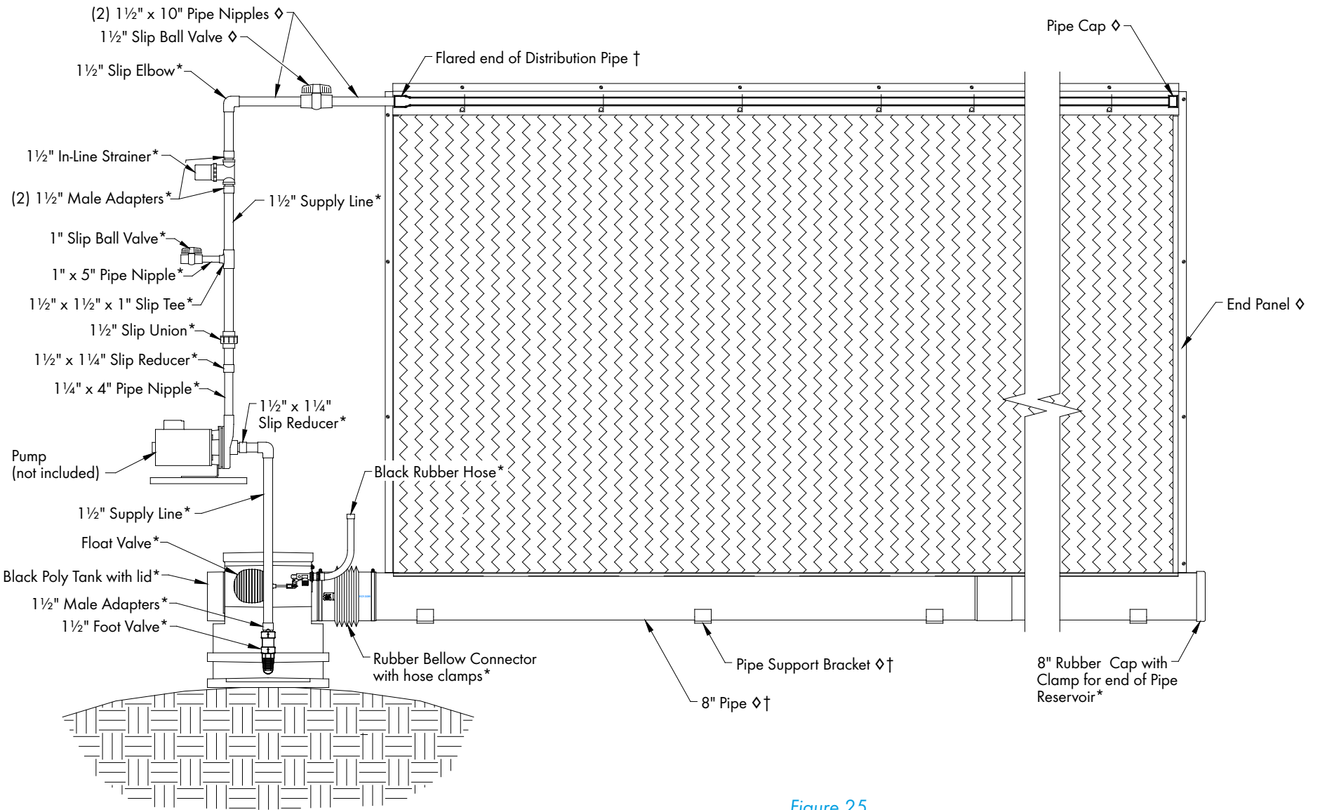
Figure 25 EC1644 BLACK POLY TANK ELEVATION VIEW WITH NON-SUBMERSIBLE PUMP
